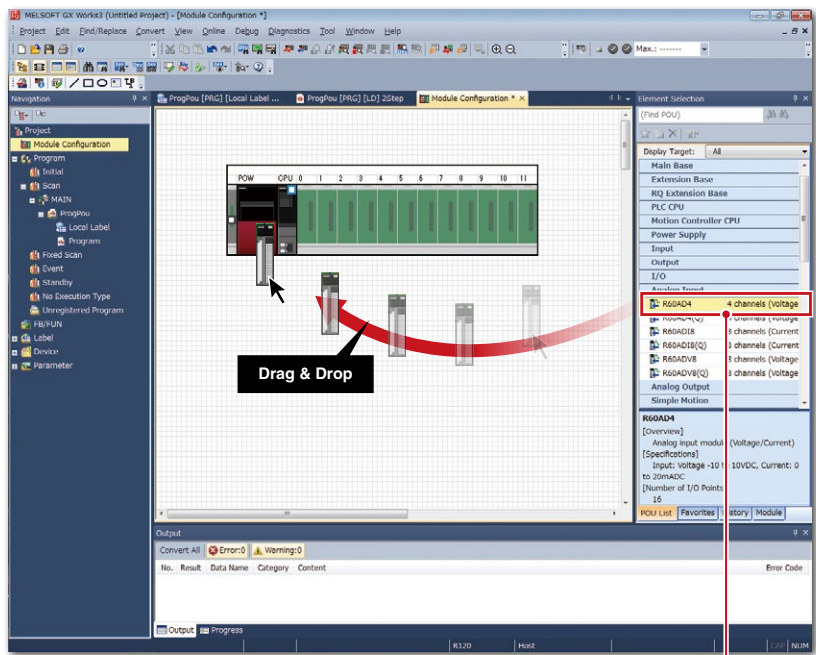
Simply drag & drop when adding a module
